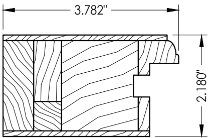
2 LATCH STILE For panel infill
