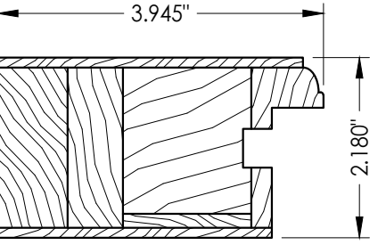
6 ASTRAGAL STILE For panel insert
