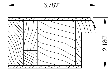
1 LATCH STILE For glass infill
