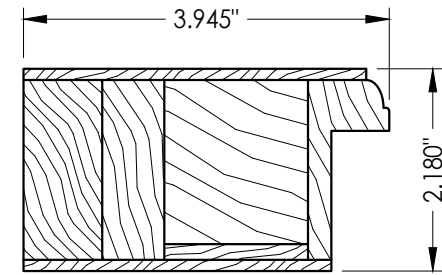
5 ASTRAGAL STILE For glass
