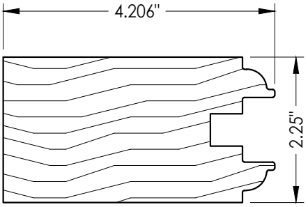
71 LATCH STILE Opaque Door
