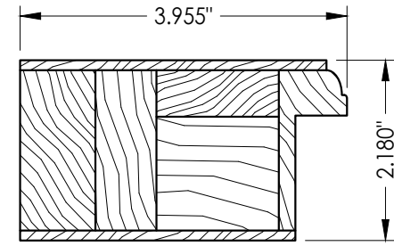
3 HINGE STILE For glass infill
