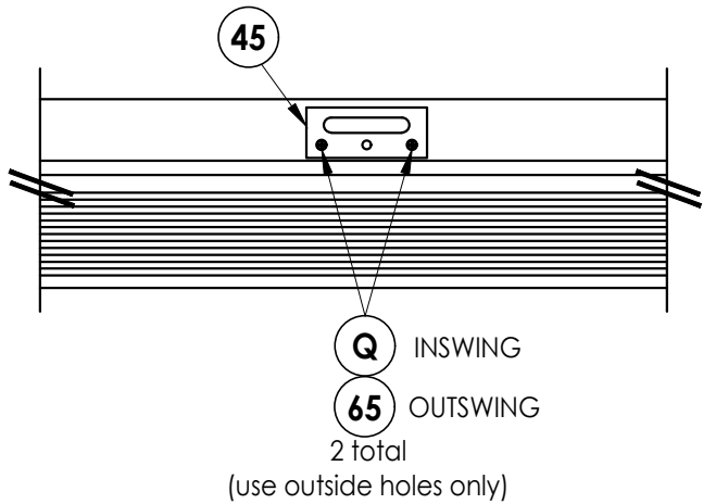
2 MULTI-POINT STRIKE INSTALLATION 9 View looking down @ sill
